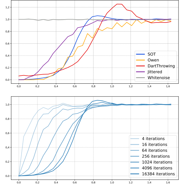
Fig. 8. 4D radial spectra. (top) Radial power spectra comparison in dimension 4 of 4K samples for various samplers; note that while dart throwing exhibits a stronger peak than SOT, its behavior at low frequencies is also significantly worse than all others (bottom) With a random initialization, the radial power spectra of SOT sampling goes from a white-noise shape to a more blue-noise one during optimization.
