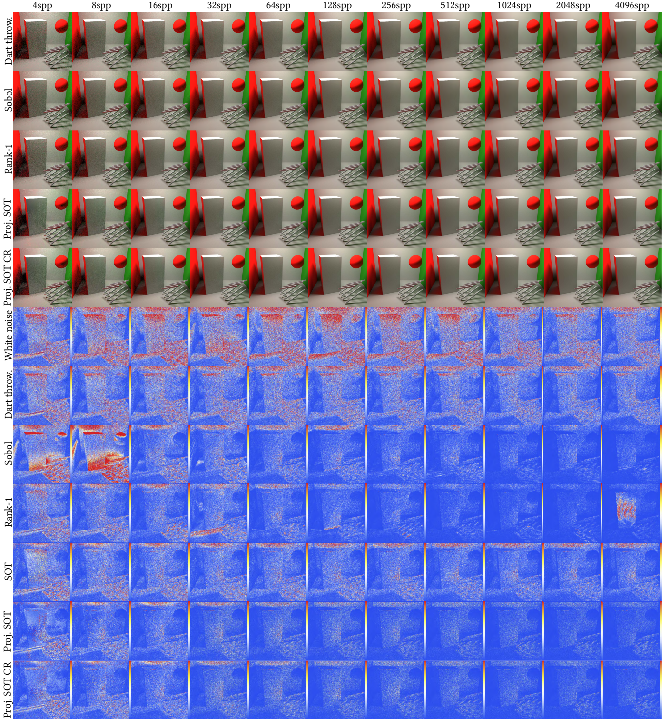
Fig. 13. Rendering results in dimension 6. We render the Cornell scene with one bounce of indirect lighting using various samplers and for several sample counts. To highlight the efficiency of Monte Carlo integrations, we display the error maps (per-pixel absolute difference with reference image in Fig. 11) using pseudocolors (from blue to red, with a linear map from 0 to 0.002/spp). While SOT sampling does not help much for rendering, its projective variant is better and/or more consistent than other typical approaches, particularly so for low counts of samples per pixel.
