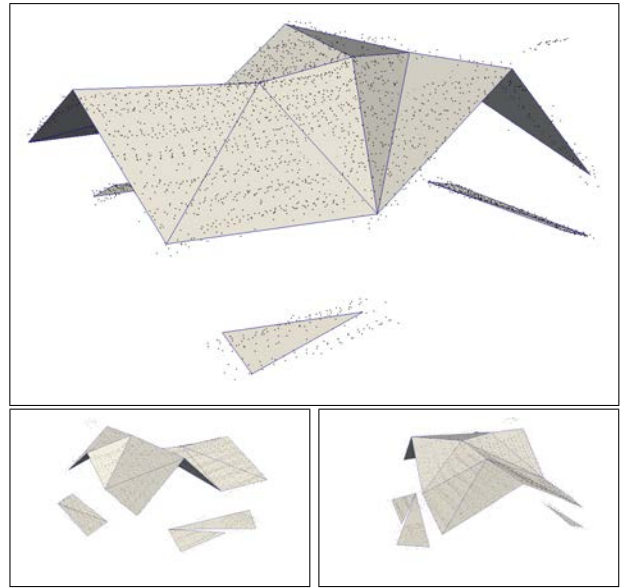
Fig. 15 Reconstruction of an aerial LIDAR point cloud capturing the rooftop of a house. Top: input point set, middle: final reconstruction, bottom: two other views. The reconstruction yields a very simplified mesh despite the noise. Point set courtesy of Qian-Yi Zhou and Ulrich Neumann.
