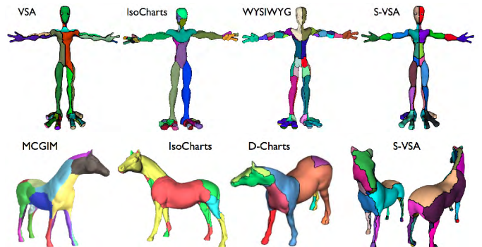
Figure 8: Comparing Chartification. Our S-VSA creates charts particularly intuitive and geometrically relevant. First row: VSA [11], IsoCharts [33], WYSIWYG [37], and S-VSA; second row: MCGIM [32], IsoCharts [33], D-Charts [34], and S-VSA.
