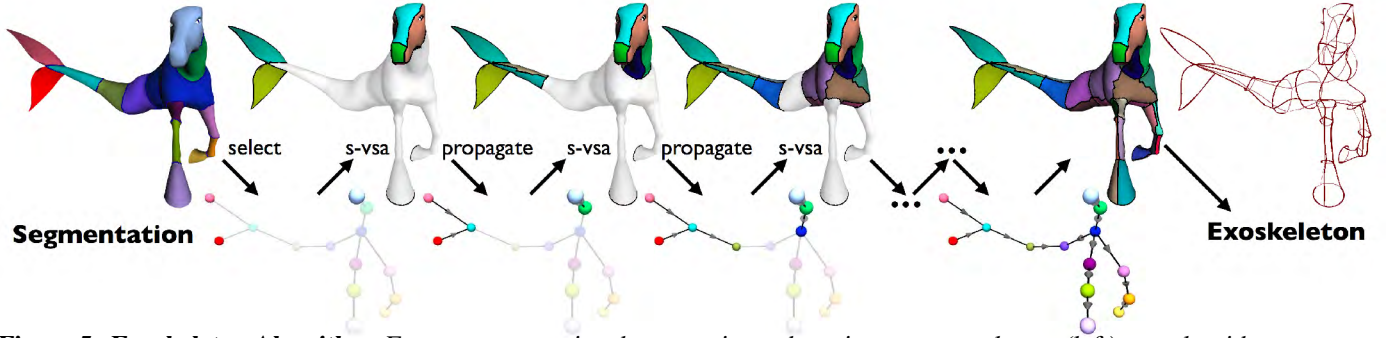
Figure 5: Exoskeleton Algorithm. From a segmentation decomposing a shape into perceptual parts (left), our algorithm constructs patches incrementally, organizing the perceptual parts in a directed graph (center). The boundaries of these patches compose a network of curves that follows perceptual and normal-based feature lines (right).
