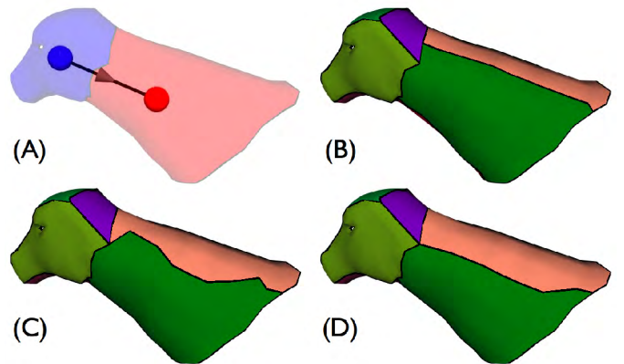
Figure 6: S-VSA. Given segmented parts (A), the VSA method [11] generates fragmented features affecting the global structure of the shape abstraction (B). Our modified S-VSA method recovers the shape structure with two simple operations: we introduce the attachment step in order to force the continuity of feature curves (C); and we extend the L^{2,1} metric based on boundary priors to favor near-orthogonal curves (D).
