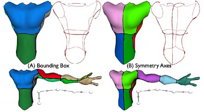
Figure 4: Select-and-Propagate. We provide a flexible mechanism to emphasize different aspects of the shape: (A) if the segmented regions are ordered from the abdomen to the hand, the resulting exoskeleton exhibits clothing seams; (B) if the order is reversed, the exoskeleton stresses symmetry axes instead.
